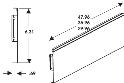
base front
