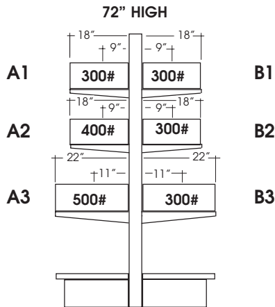
EVENLY LOADED SHELVES ON ISLANDS
