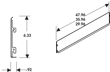
flush base
