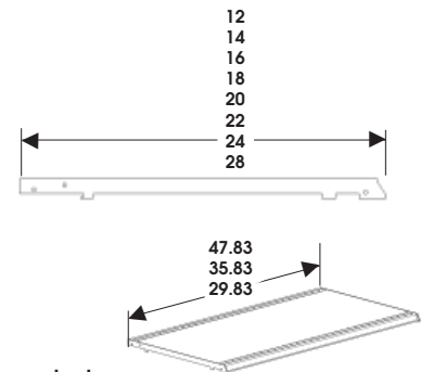
base deck
