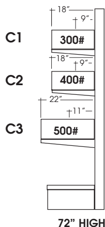
EVENLY LOADED SHELVES ON WALL UNITS
